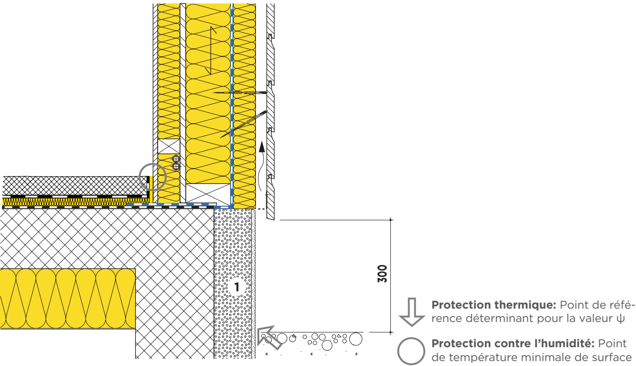
1 Panneau XPS, \lambda_D = 0.034 \text{ W/(m K)}
